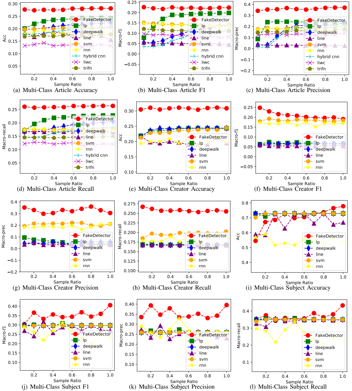
Fig. 7. Multi-Class Credibility Inference of News Articles 7(a)-7(d), Creators 7(e)-7(h) and Subjects 7(i)-7(l).
