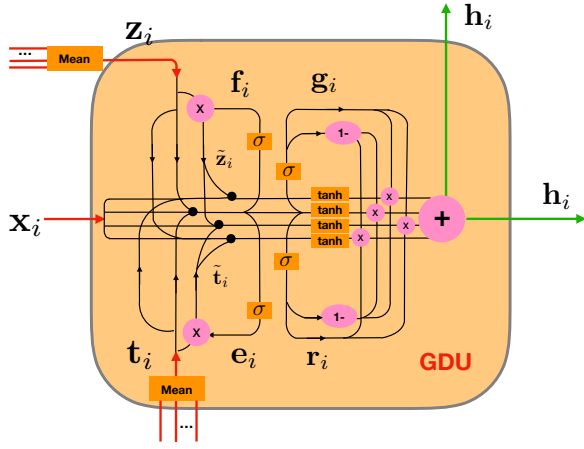
Fig. 4. Gated Diffusive Unit (GDU).
