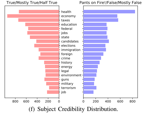
Fig. 1. PolitiFact Dataset Statistical Analysis. (Plots (a)-(b): frequent words used in true/fake news articles; Plots (c)-(d): credibility of news articles from the Republican and the Democratic; Plots (e)-(f): some basic statistical information of the dataset.)
