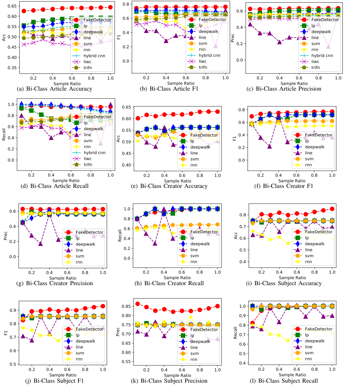
Fig. 6. Bi-Class Credibility Inference of News Articles 6(a)-6(d), Creators 6(e)-6(h) and Subjects 6(i)-6(l).
